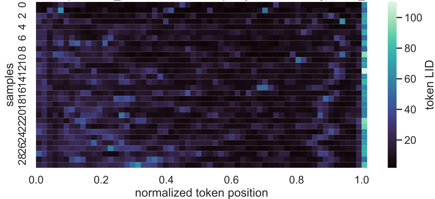
1.7B Exp C think_answer LID heatmap, layer 6, sorted by mean_lid
