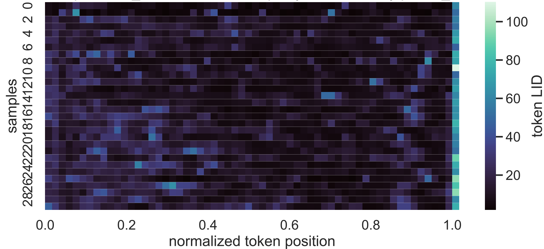
1.7B Exp C think_answer LID heatmap, layer 6, sorted by paired_delta
