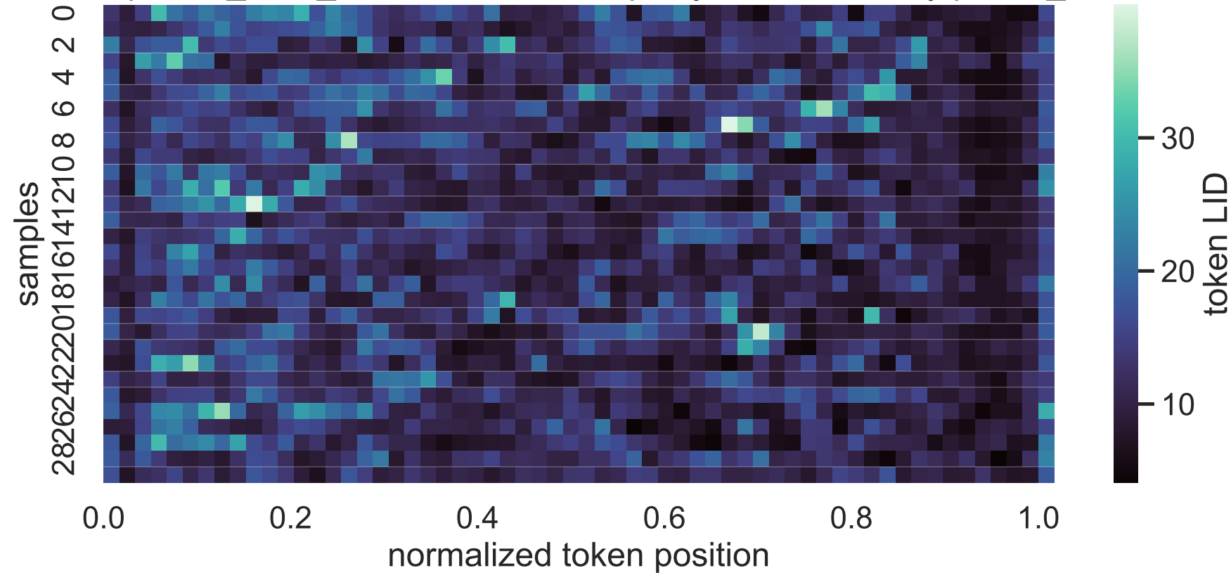
14B Exp C no_think_answer LID heatmap, layer 20, sorted by paired_delta
