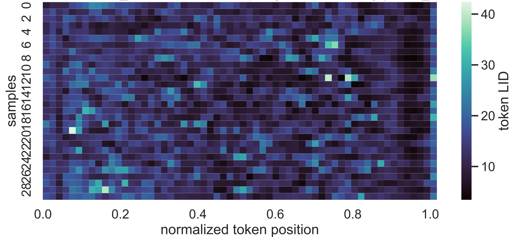
14B Exp C think_answer LID heatmap, layer 20, sorted by paired_delta
