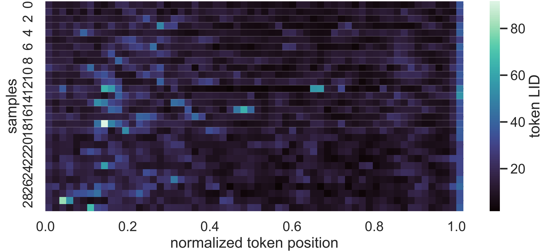
32B Exp C no_think_answer LID heatmap, layer 13, sorted by correctness_then_mean_lid
