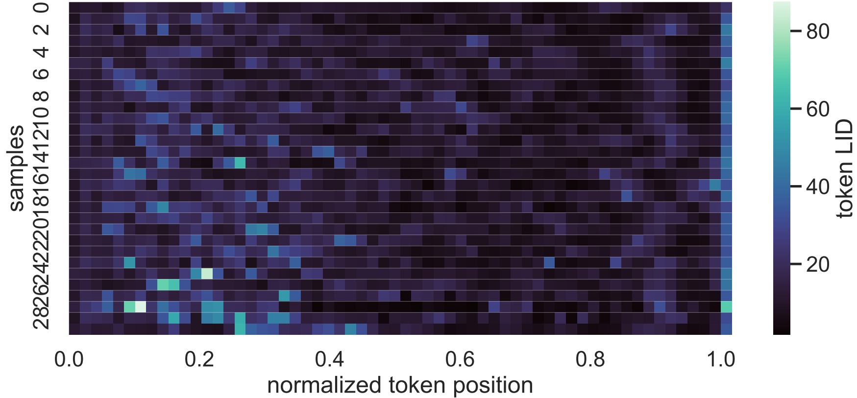
32B Exp C think_answer LID heatmap, layer 13, sorted by correctness_then_mean_lid
