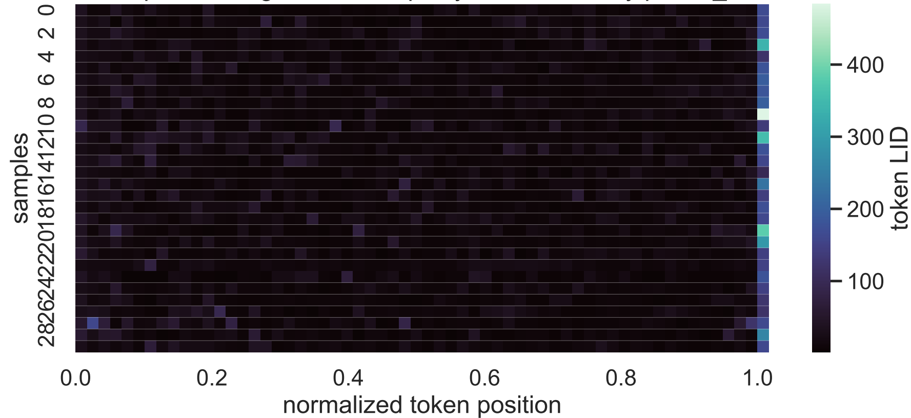
32B Exp C thinking LID heatmap, layer 13, sorted by paired_delta
