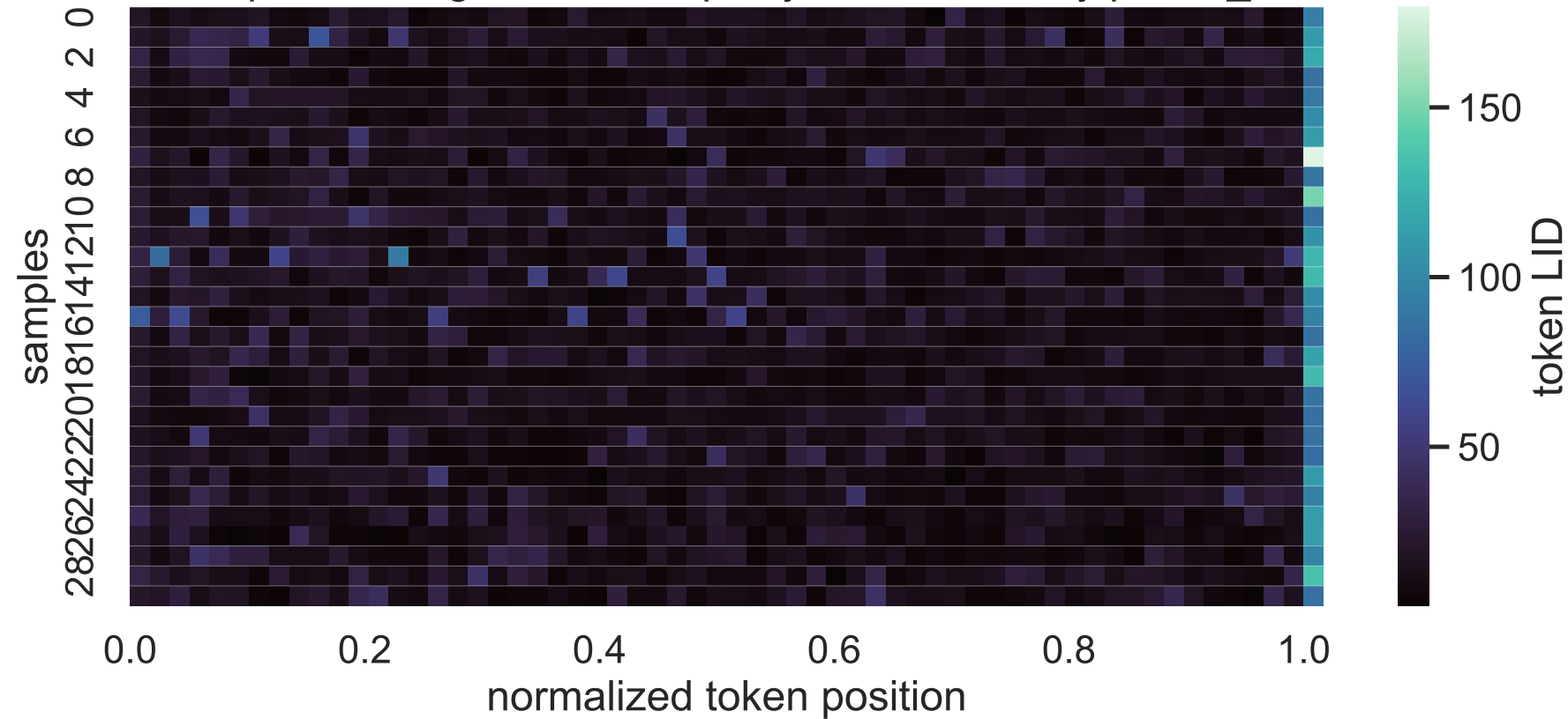
32B Exp C thinking LID heatmap, layer 20, sorted by paired_delta
