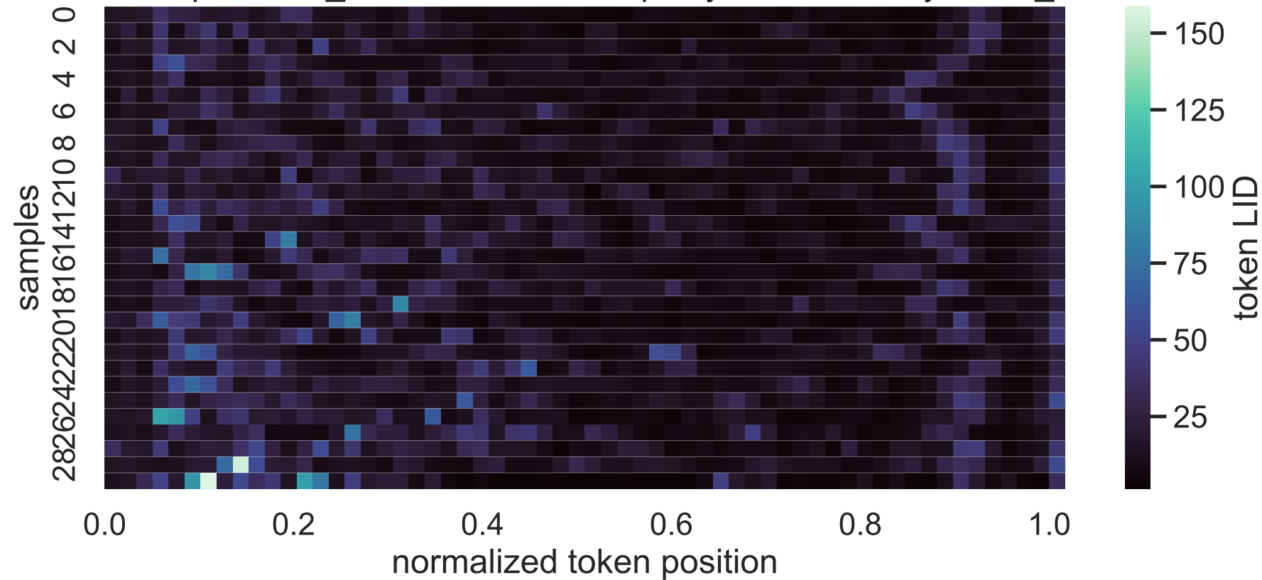
32B Exp C think_answer LID heatmap, layer 6, sorted by mean_lid
