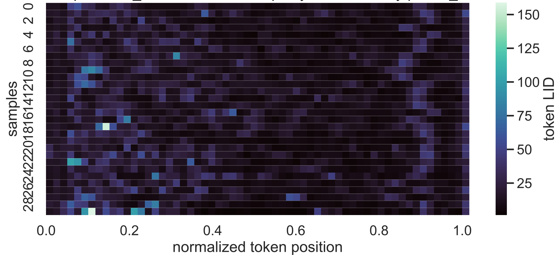
32B Exp C think_answer LID heatmap, layer 6, sorted by paired_delta
