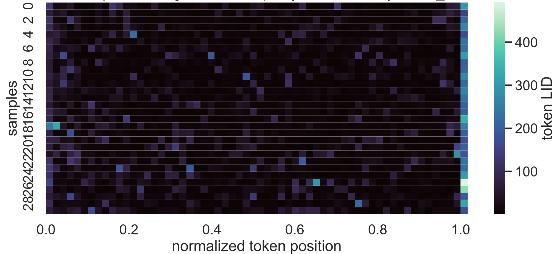
32B Exp C thinking LID heatmap, layer 6, sorted by mean_lid
