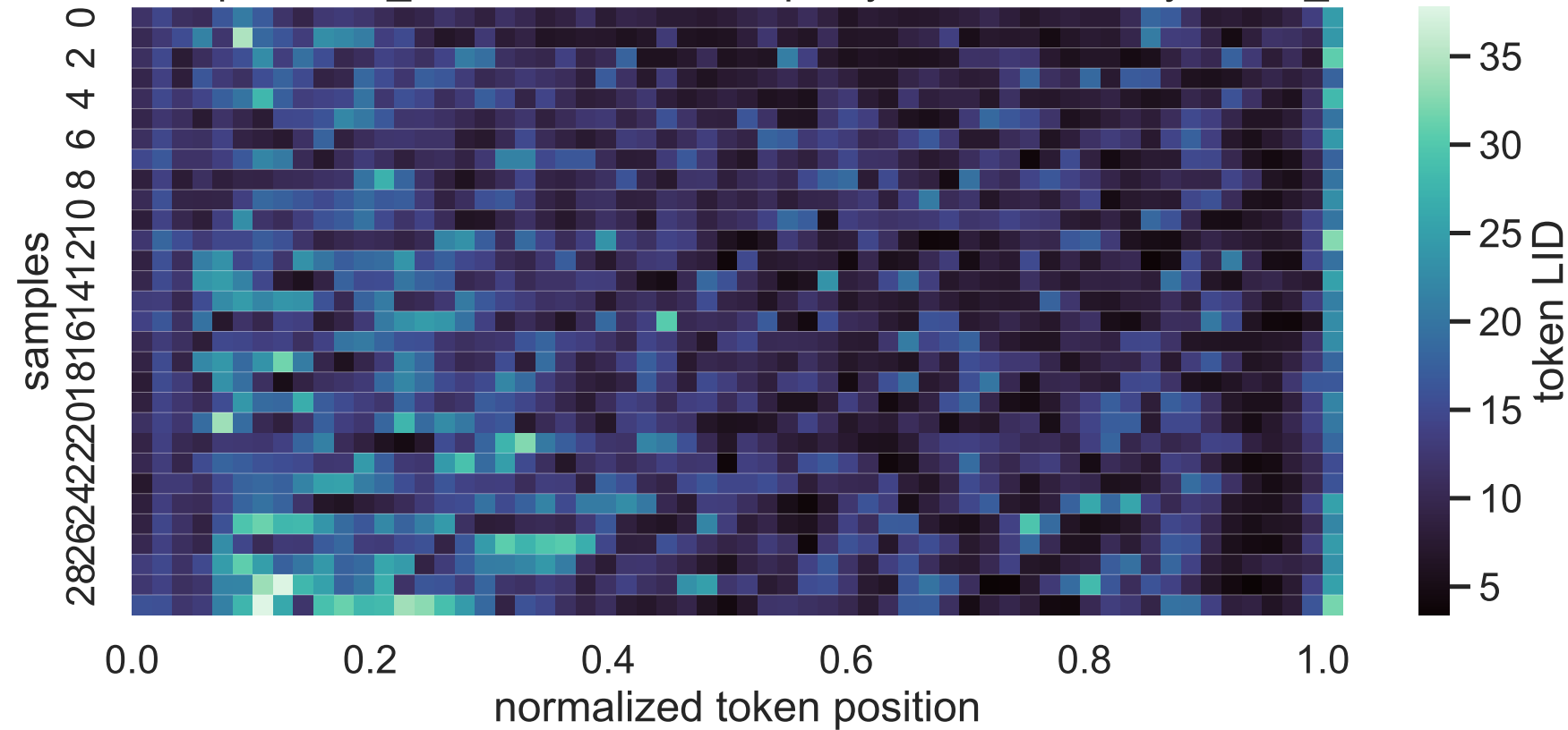
8B Exp C think_answer LID heatmap, layer 13, sorted by mean_lid
