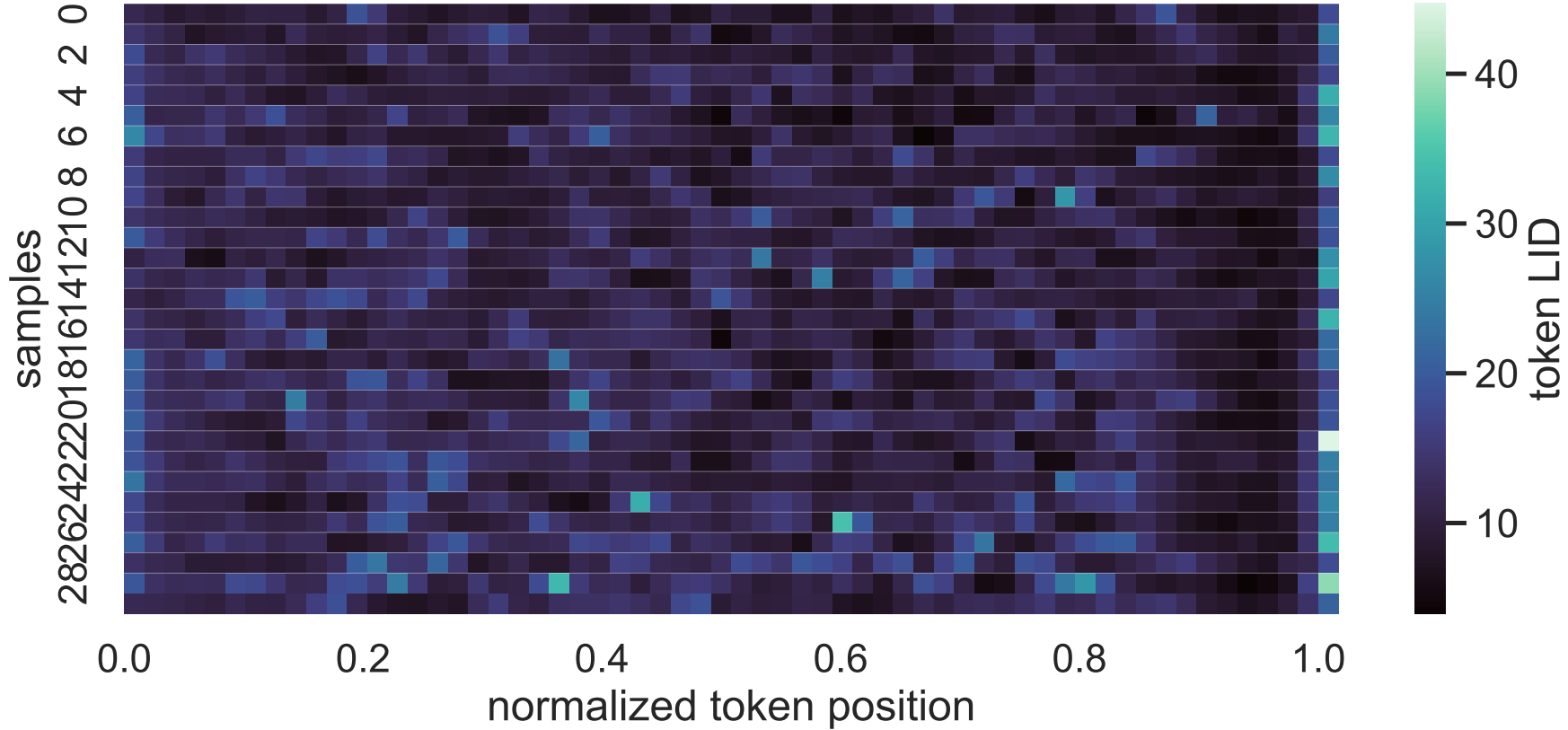
8B Exp C think_answer LID heatmap, layer 20, sorted by correctness_then_mean_lid
