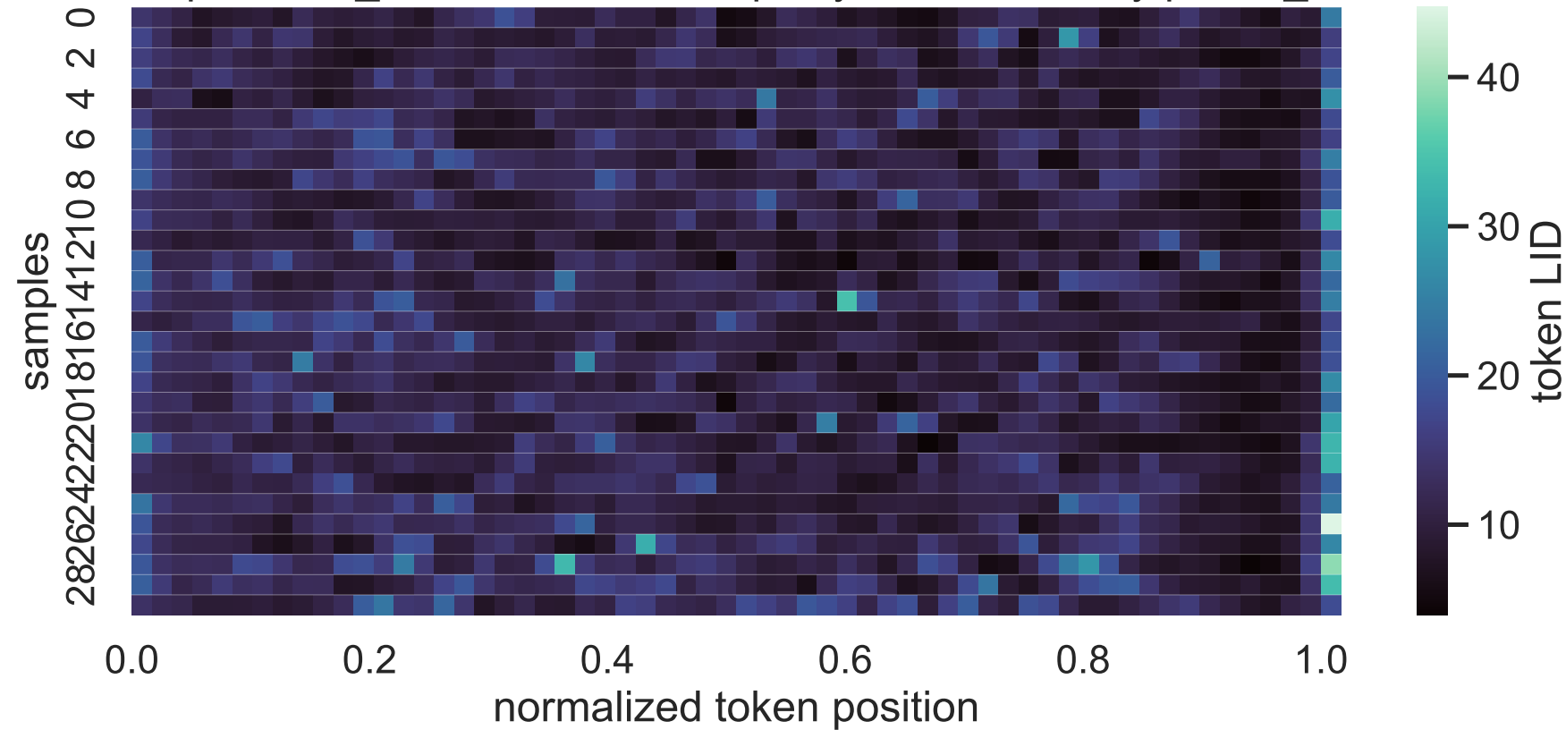
8B Exp C think_answer LID heatmap, layer 20, sorted by paired_delta
