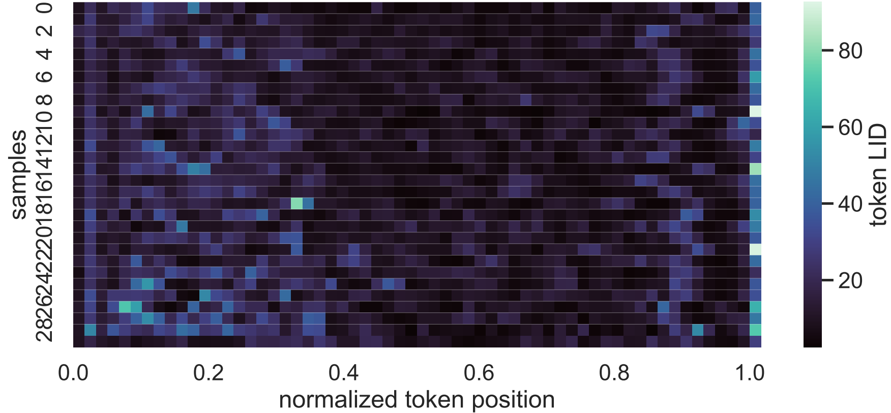
8B Exp C think_answer LID heatmap, layer 6, sorted by correctness_then_mean_lid
