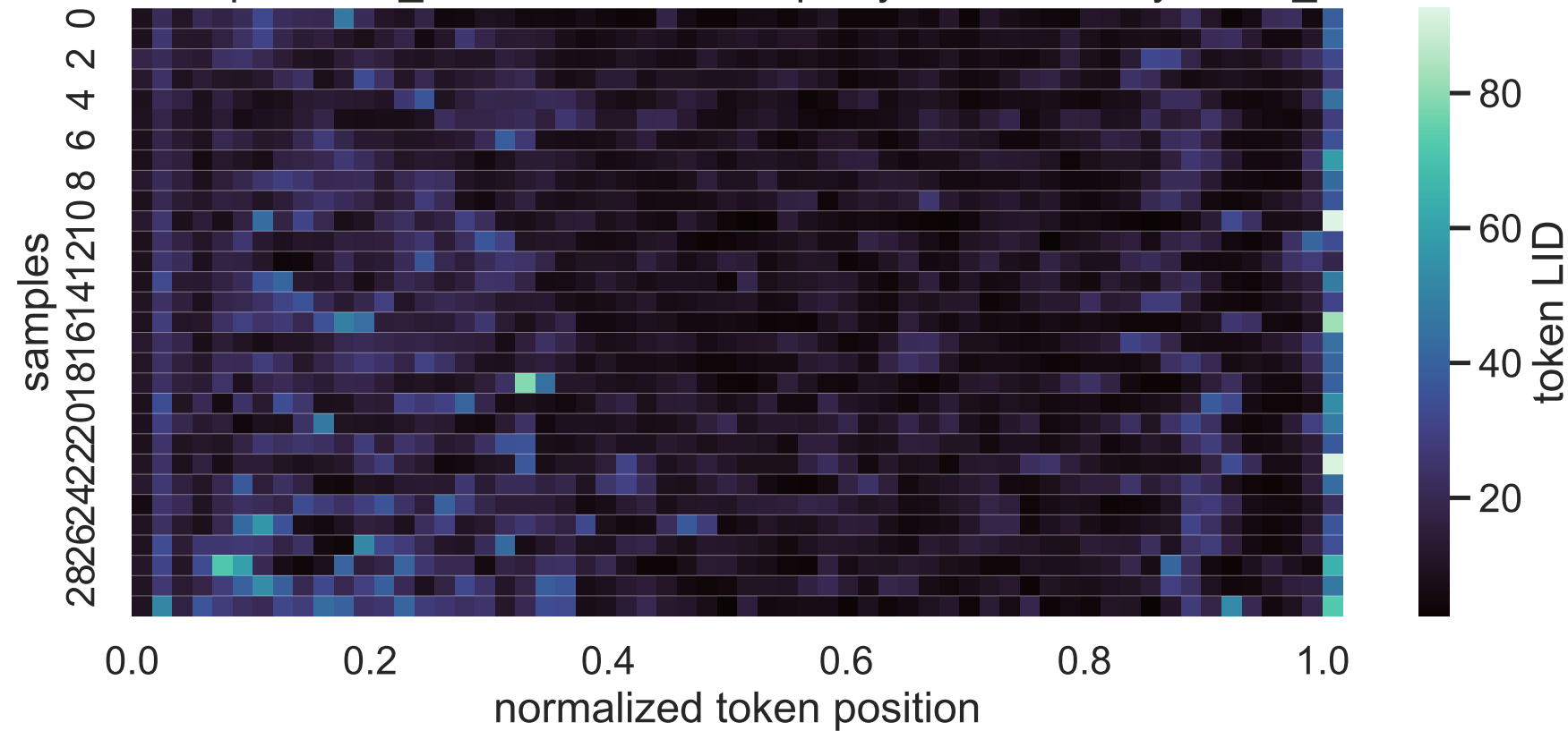
8B Exp C think_answer LID heatmap, layer 6, sorted by mean_lid
