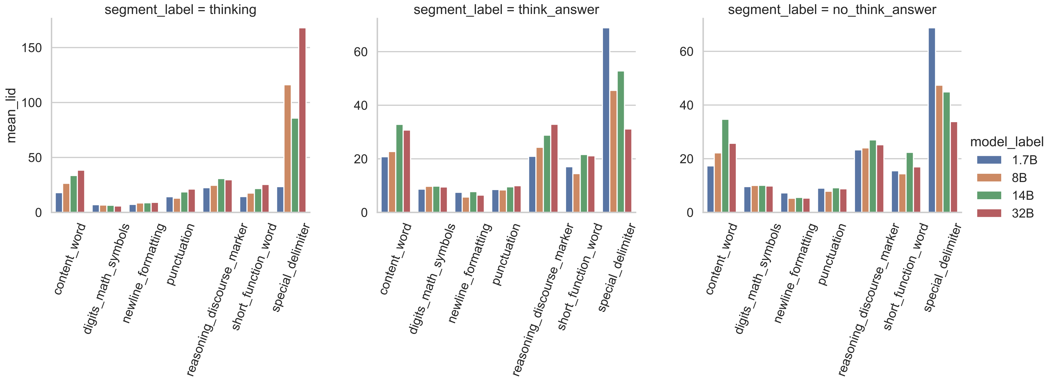
Exp C token-category mean LID, layer 6
