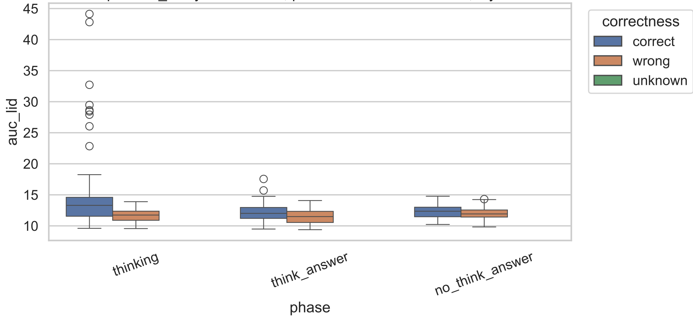
Exp C auc_lid by correctness, pooled across model sizes, layer 20
