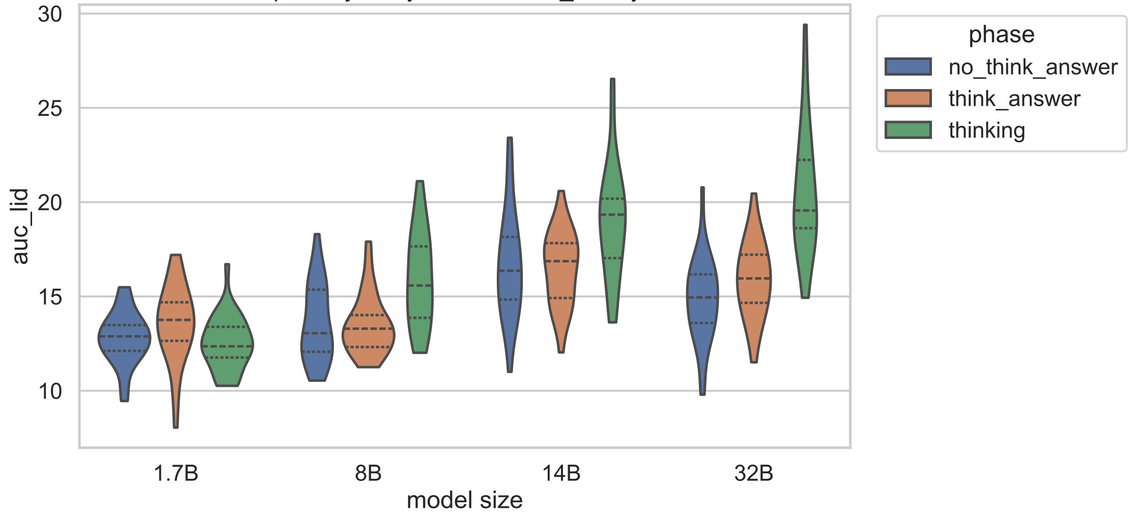
Exp C trajectory statistic: auc_lid, layer 6
