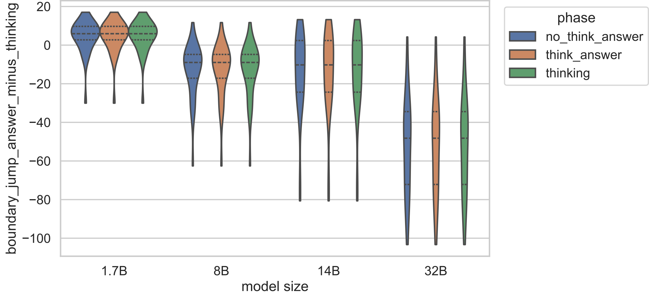
Exp C trajectory statistic: boundary_jump_answer_minus_thinking, layer 6
