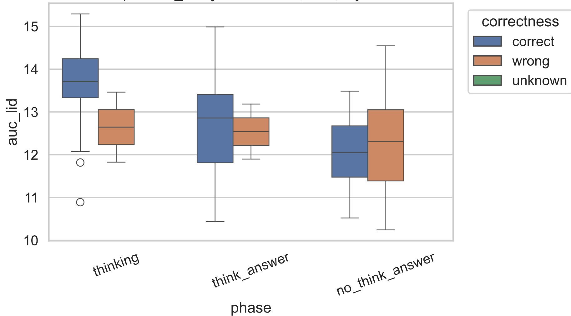
Exp C auc_lid by correctness, 14B, layer 13
