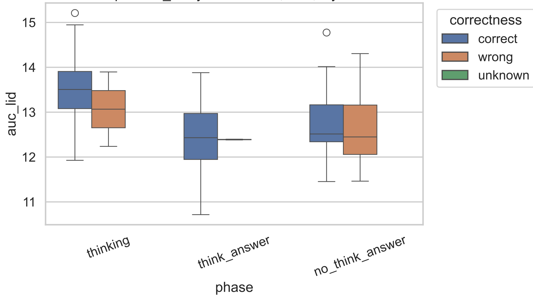
Exp C auc_lid by correctness, 14B, layer 20
