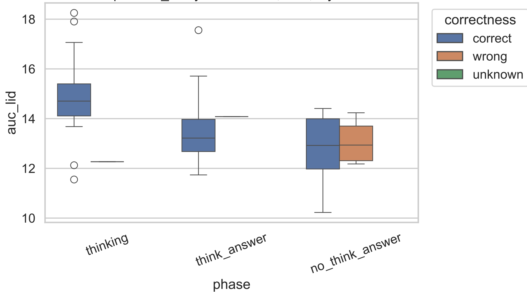
Exp C auc_lid by correctness, 32B, layer 20
