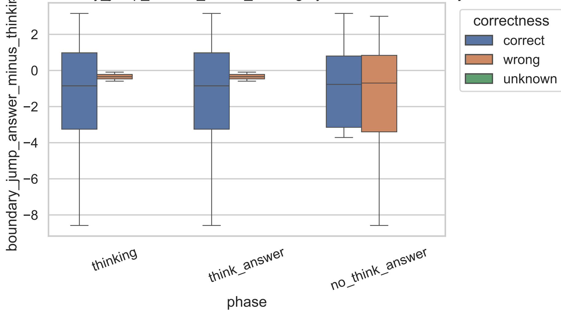
Exo C boundary_jump_answer_minus_thinking by correctness, 14B, layer 20
