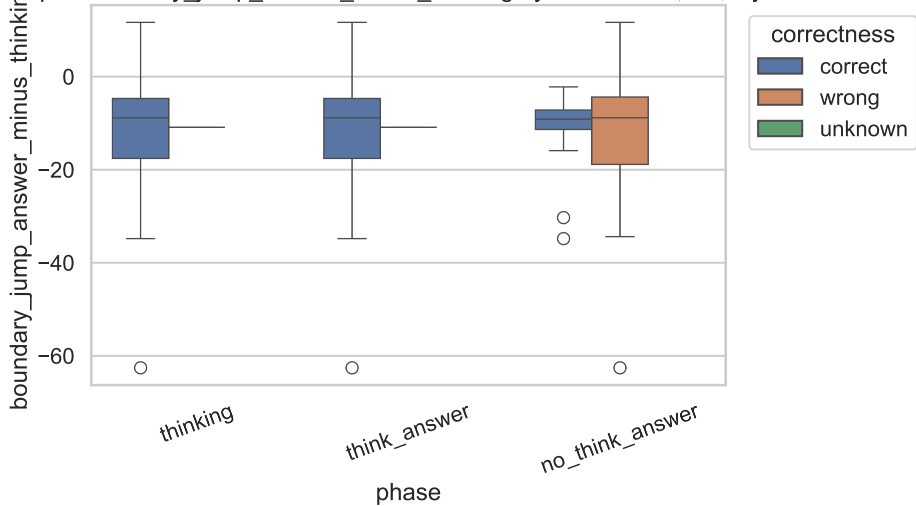
exp C boundary_jump_answer_minus_thinking by correctness, 8B, layer 6
