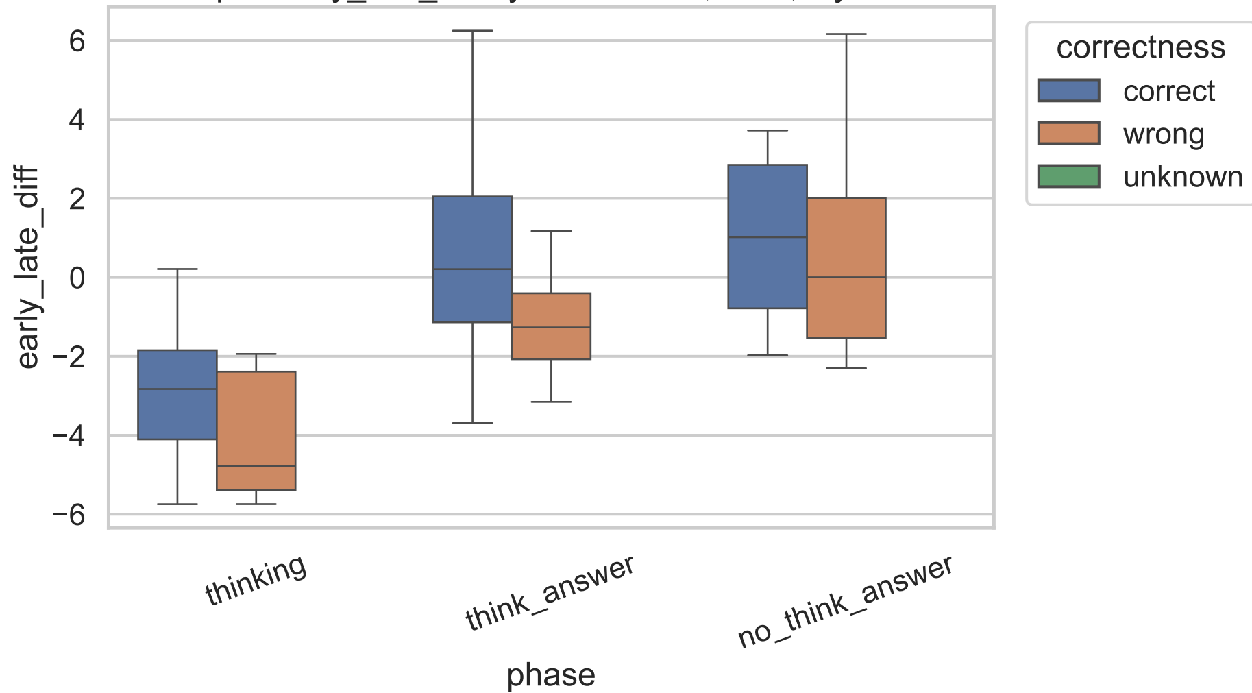
Exp C early_late_diff by correctness, 1.7B, layer 20
