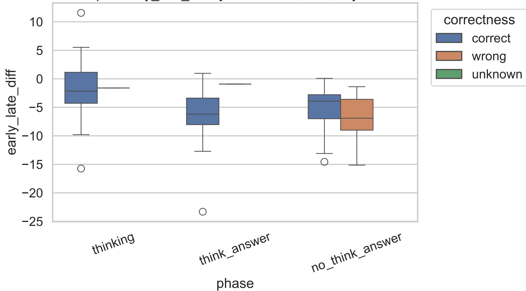
Exp C early_late_diff by correctness, 32B, layer 13
