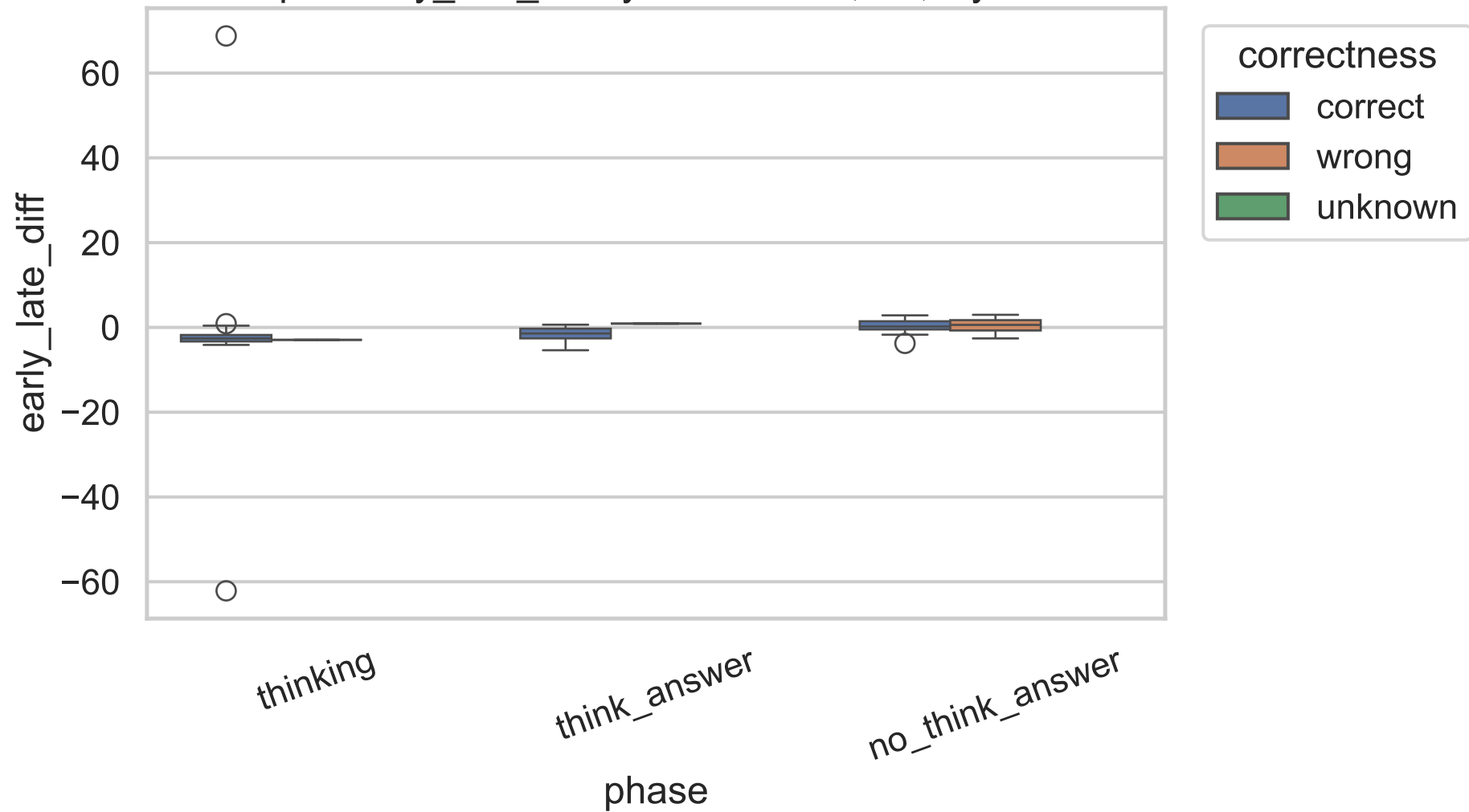
Exp C early_late_diff by correctness, 8B, layer 20
