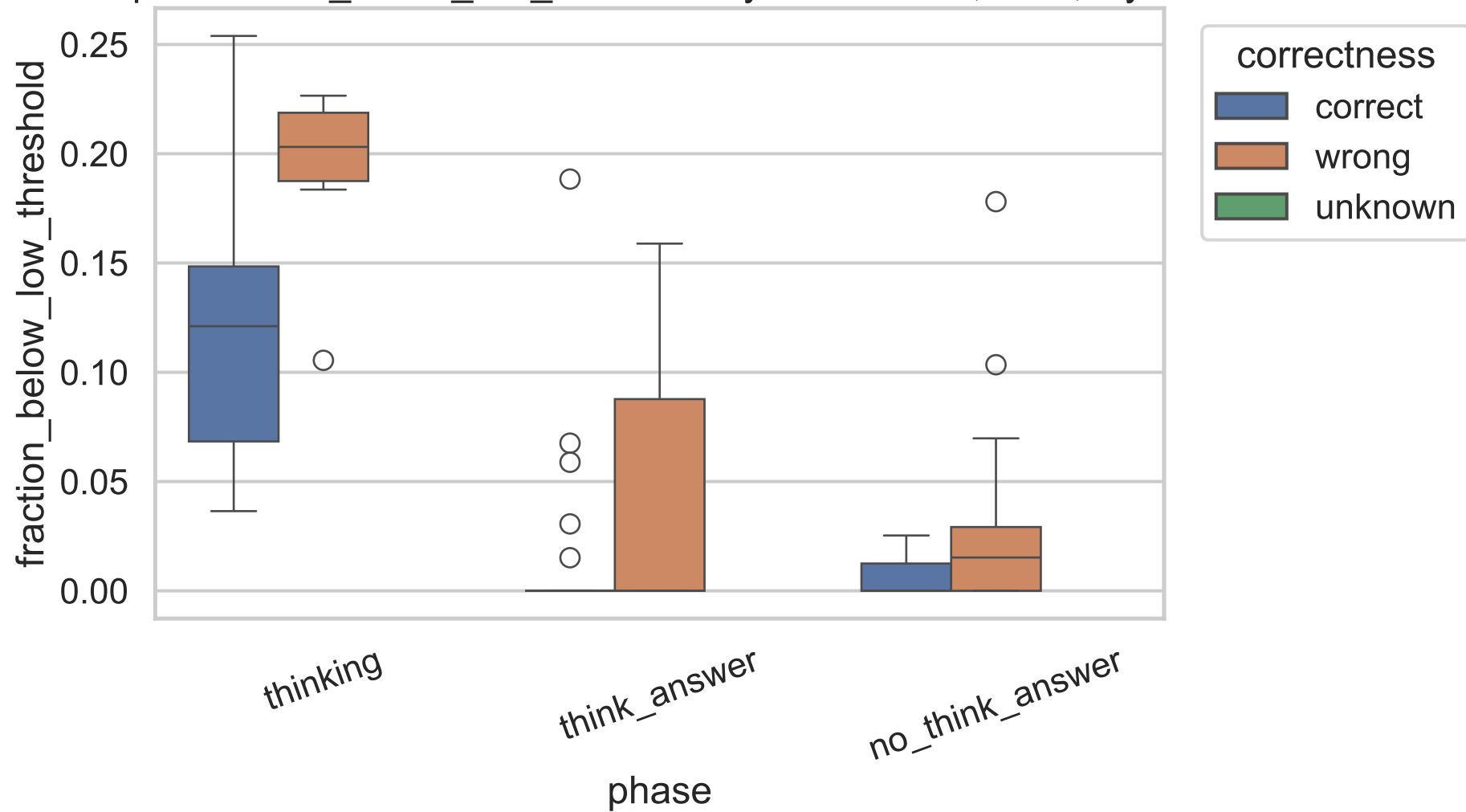
Exp C fraction_below_low_threshold by correctness, 1.7B, layer 13
