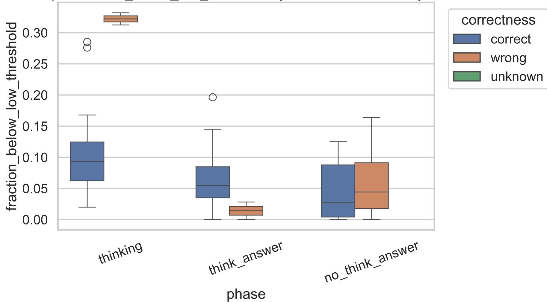
Exp C fraction_below_low_threshold by correctness, 14B, layer 13
