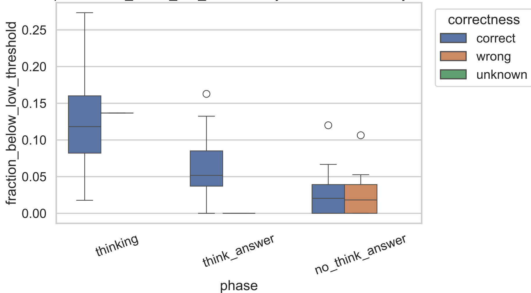
Exp C fraction_below_low_threshold by correctness, 8B, layer 20
