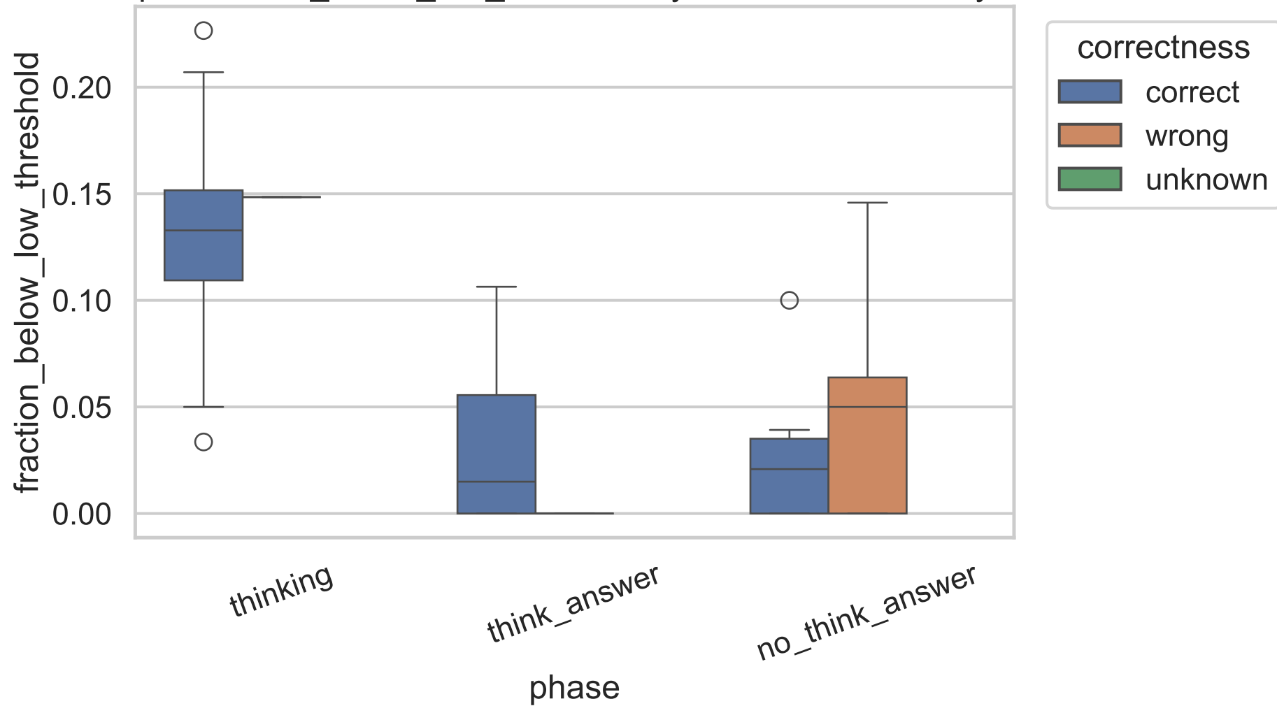
Exp C fraction_below_low_threshold by correctness, 8B, layer 6
