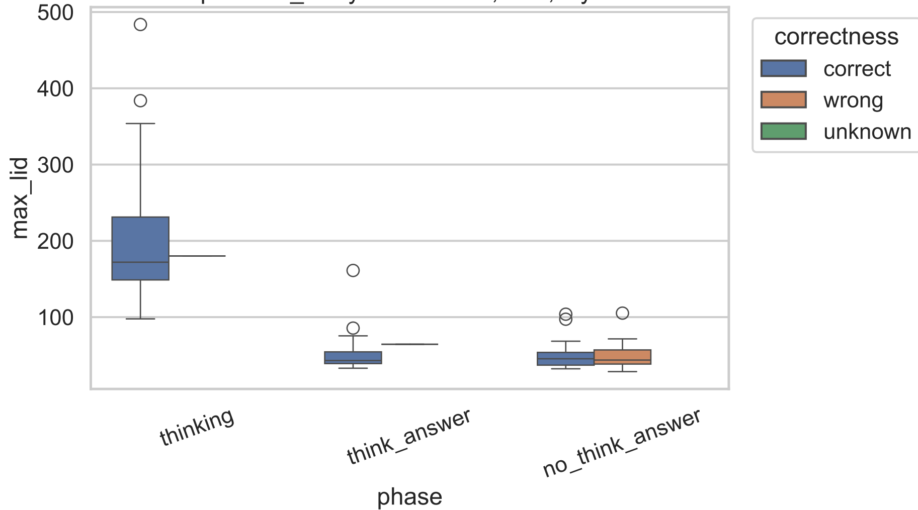
Exp C max_lid by correctness, 32B, layer 13
