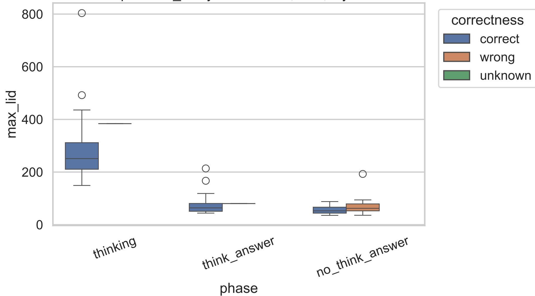
Exp C max_lid by correctness, 32B, layer 6
