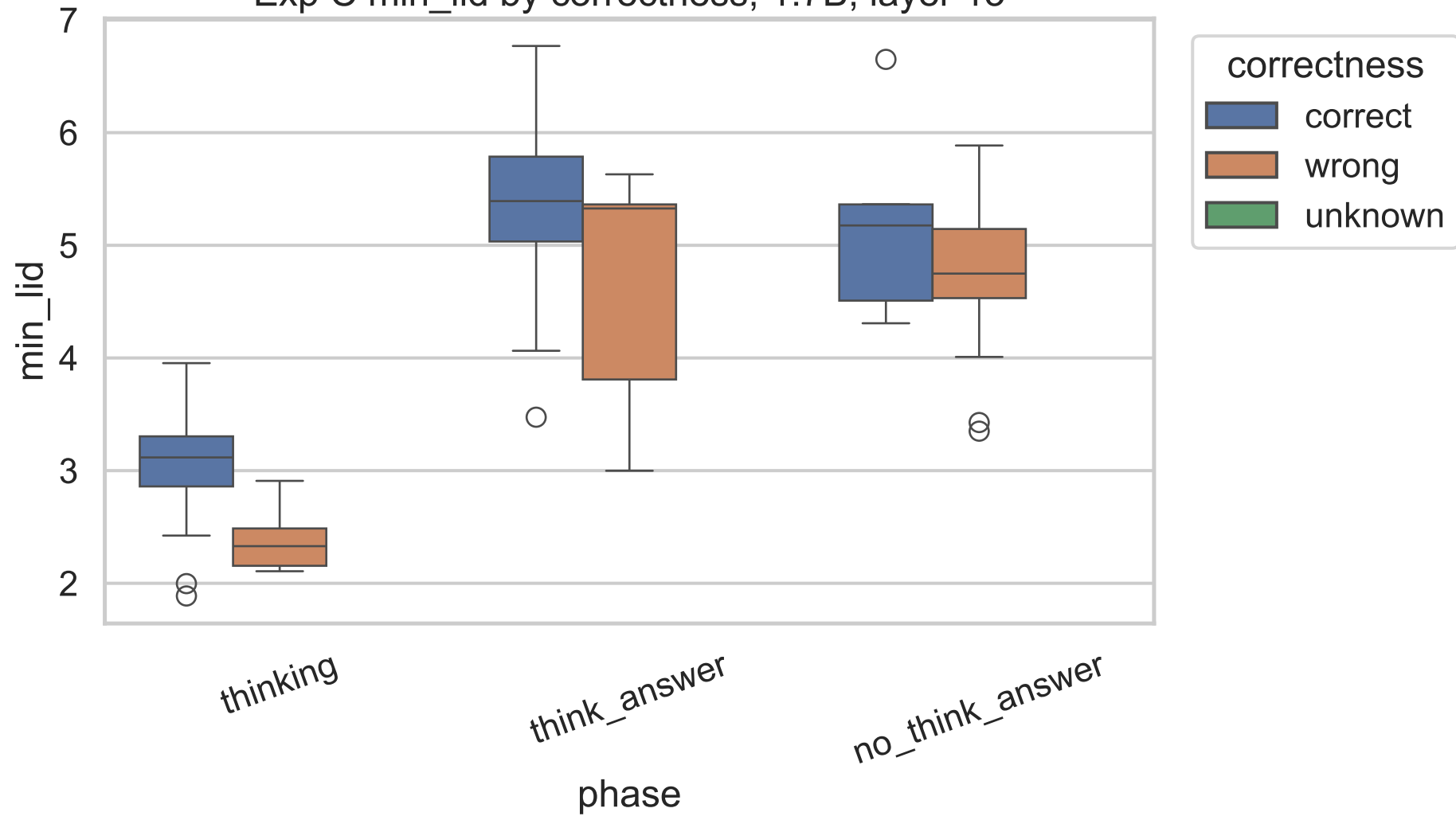
Exp C min_lid by correctness, 1.7B, layer 13
