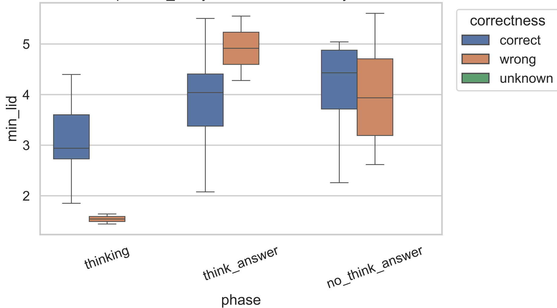
Exp C min_lid by correctness, 14B, layer 13
