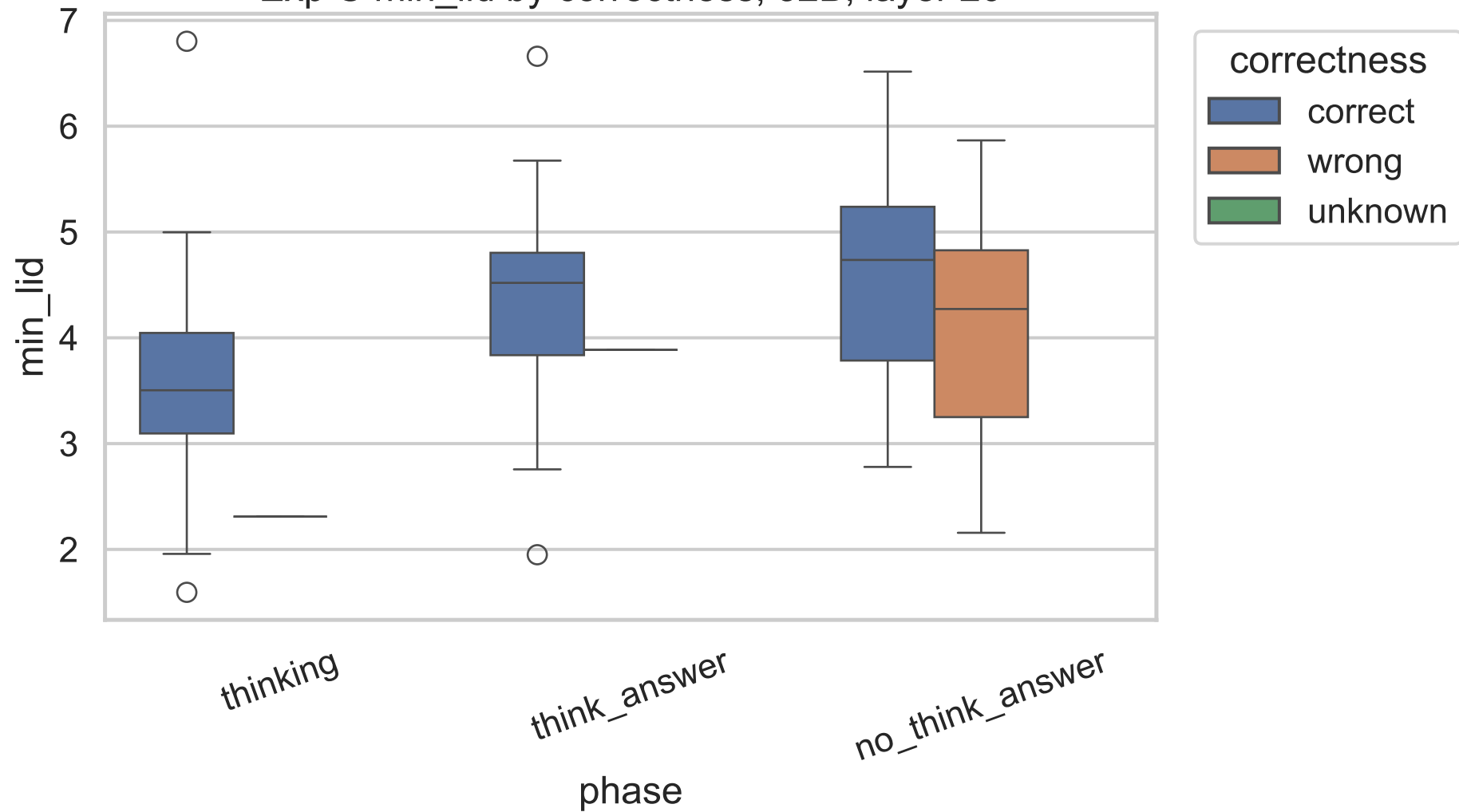
Exp C min_lid by correctness, 32B, layer 20
