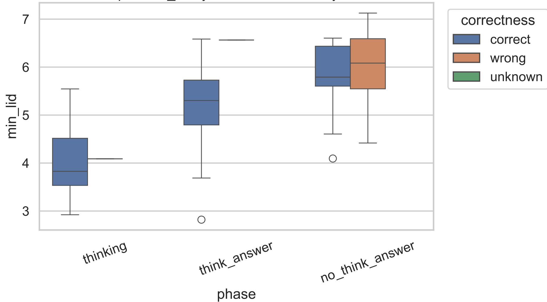
Exp C min_lid by correctness, 8B, layer 20
