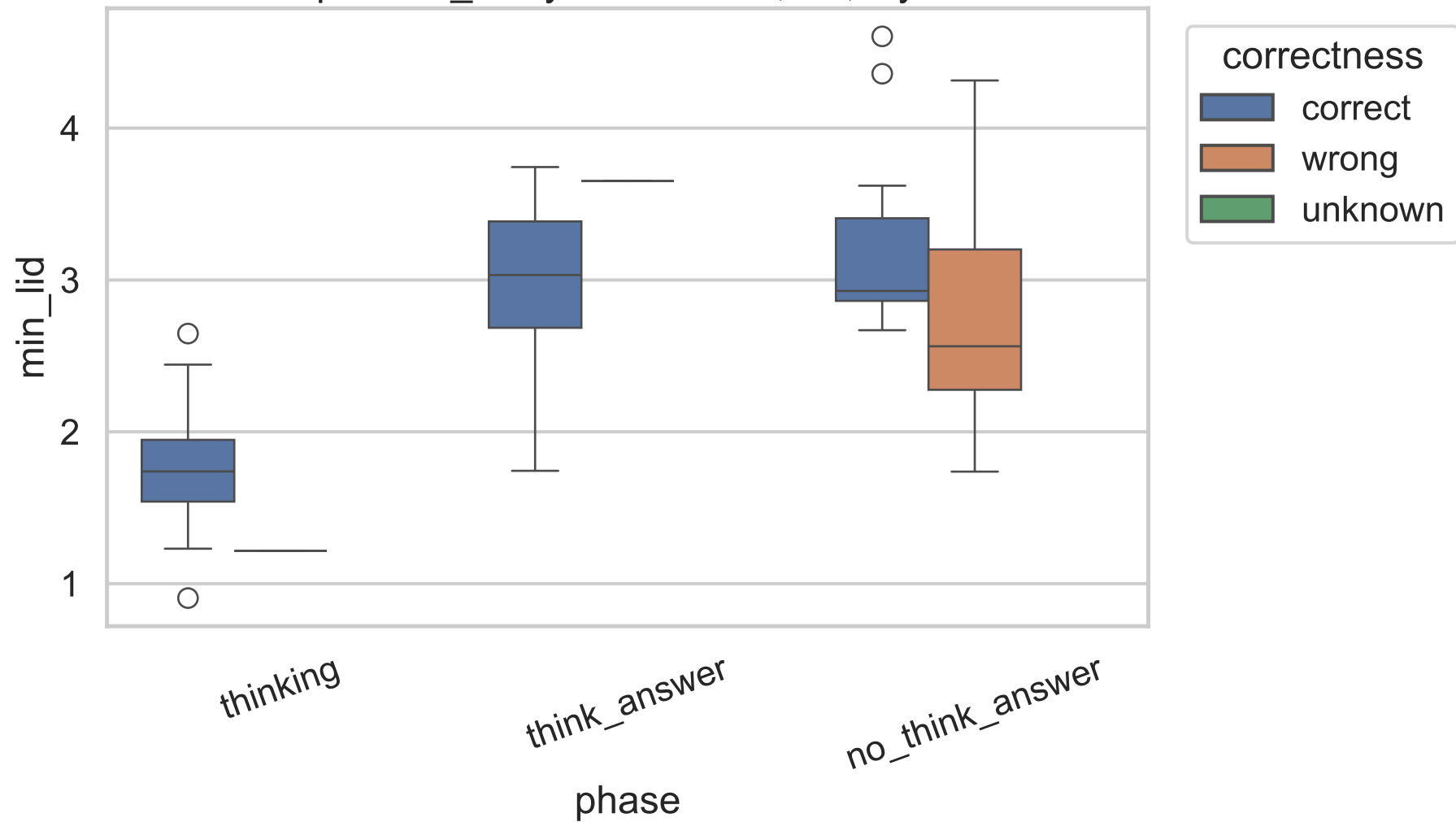
Exp C min_lid by correctness, 8B, layer 6
