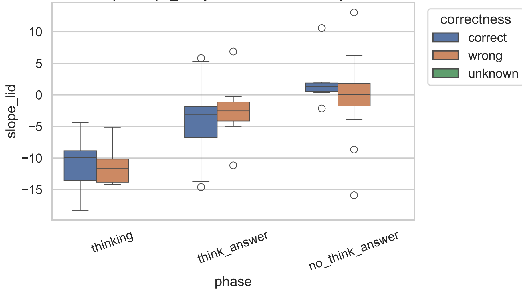
Exp C slope_lid by correctness, 1.7B, layer 6
