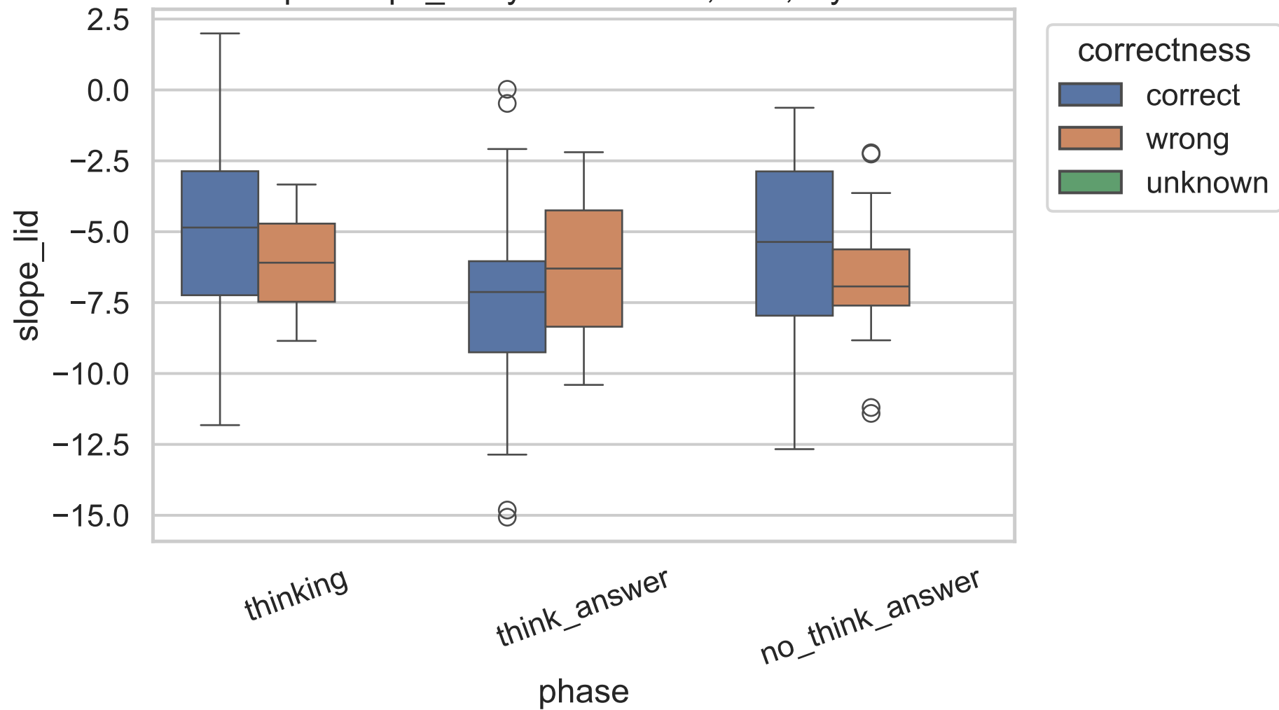
Exp C slope_lid by correctness, 14B, layer 13
