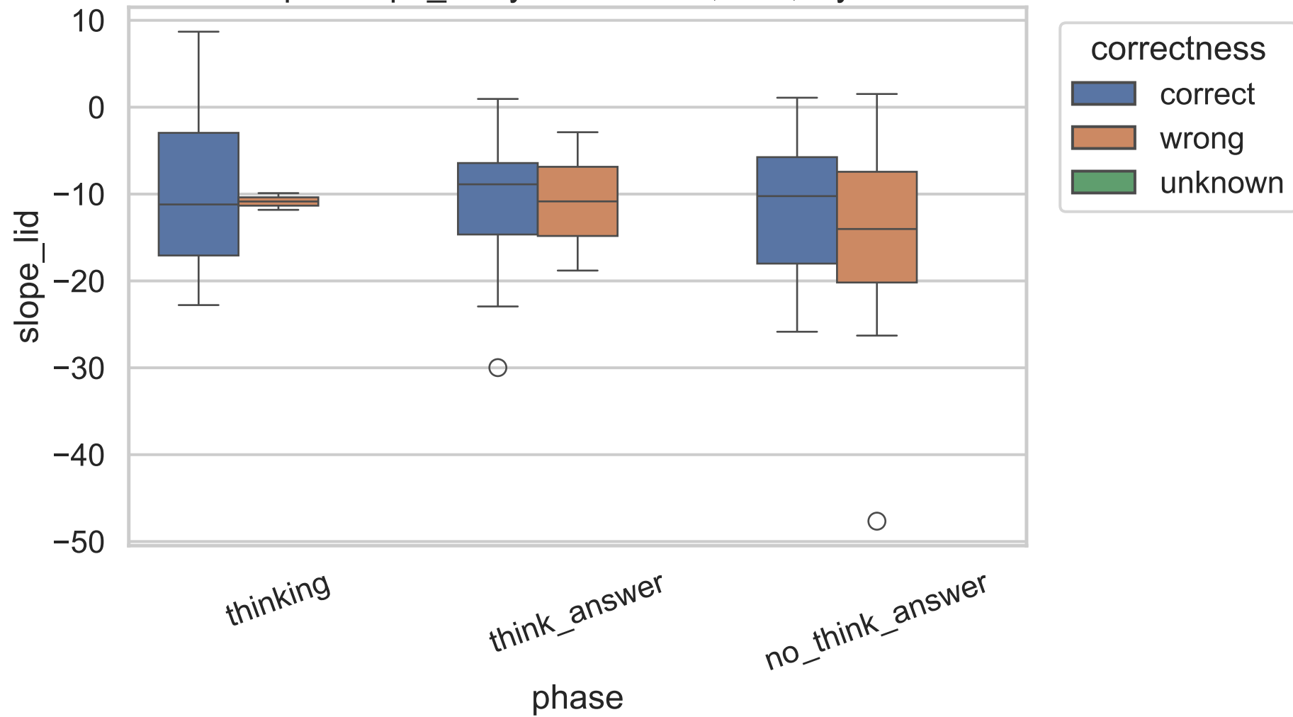
Exp C slope_lid by correctness, 14B, layer 6
