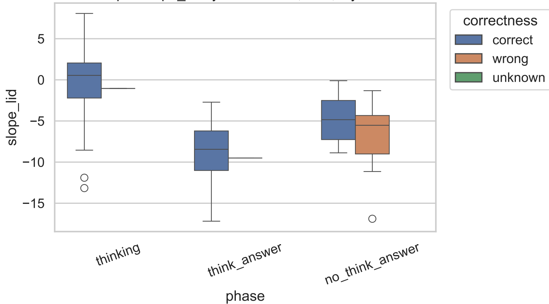
Exp C slope_lid by correctness, 32B, layer 20
