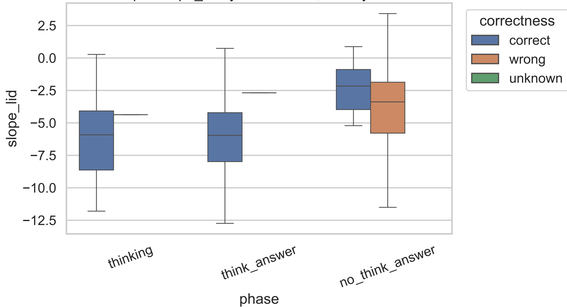
Exp C slope_lid by correctness, 8B, layer 13
