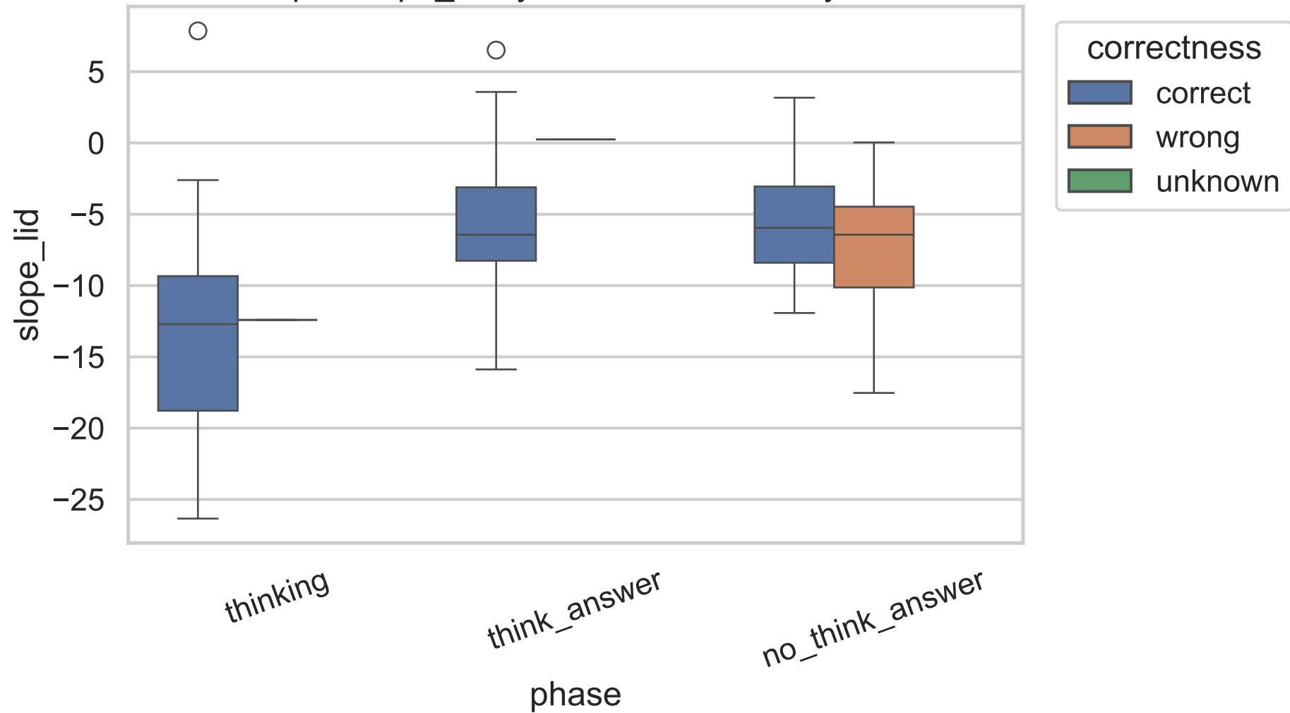
Exp C slope_lid by correctness, 8B, layer 6
