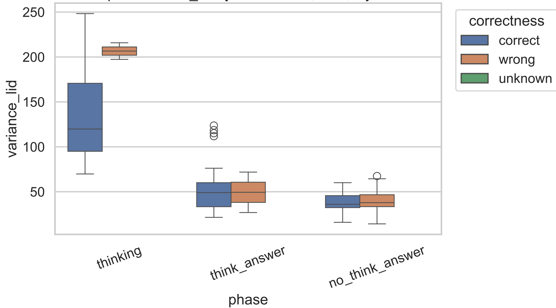
Exp C variance_lid by correctness, 14B, layer 13
