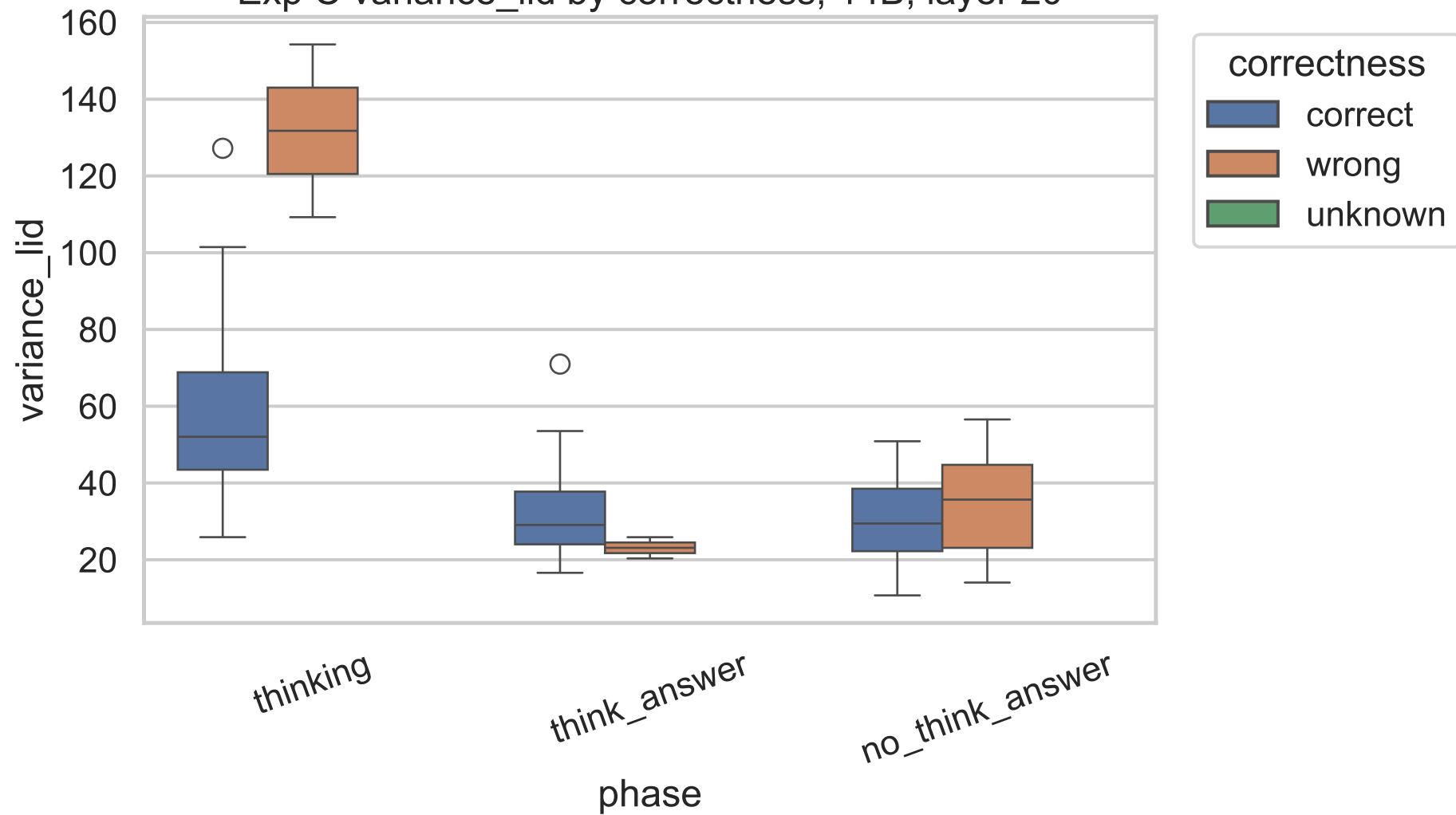
Exp C variance_lid by correctness, 14B, layer 20
