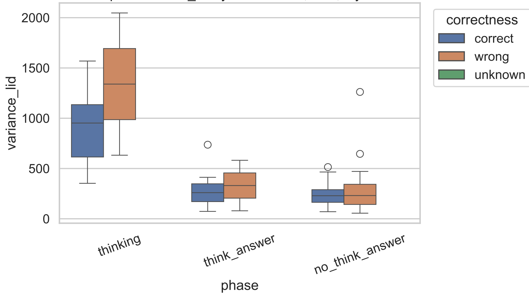
Exp C variance_lid by correctness, 14B, layer 6
