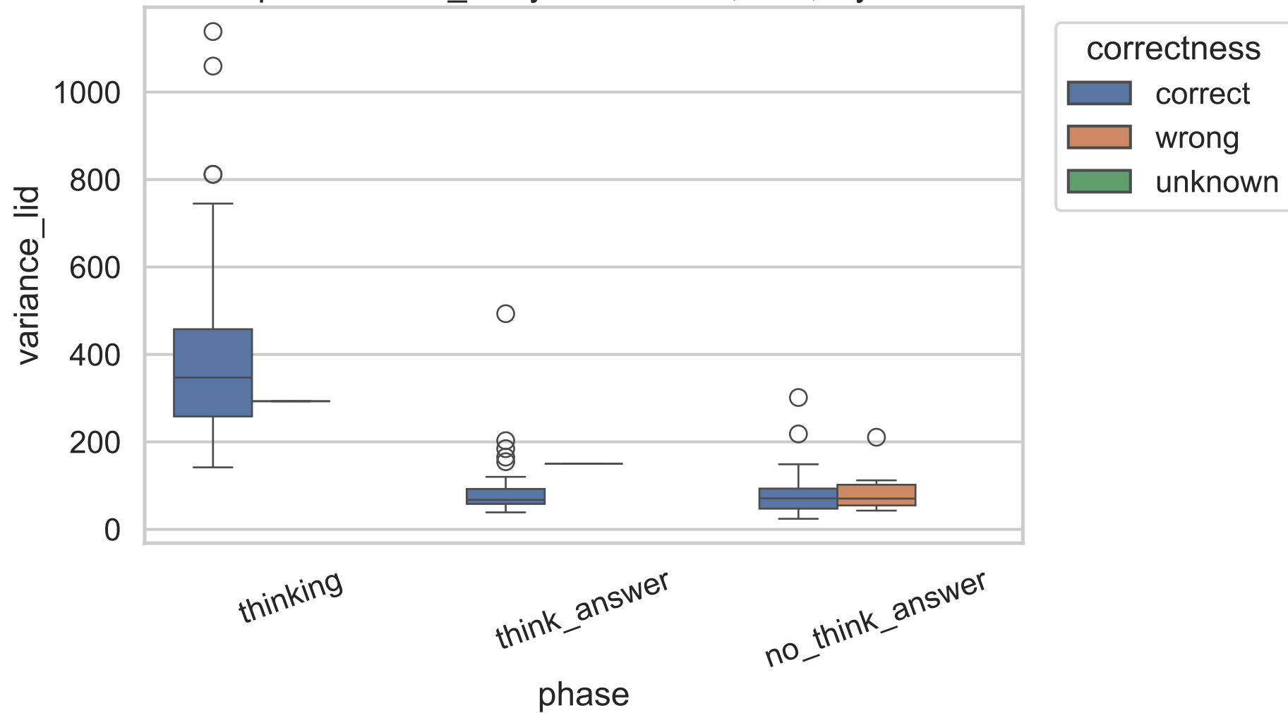
Exp C variance_lid by correctness, 32B, layer 13
