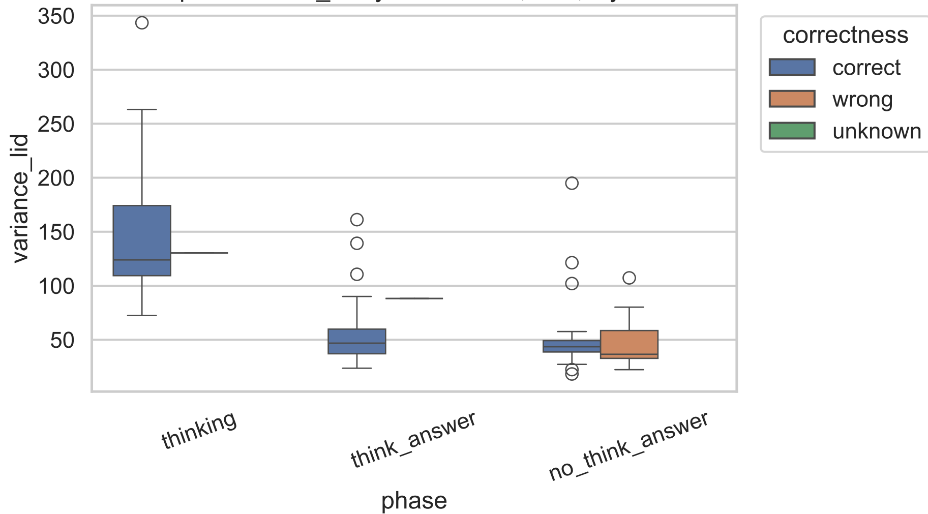
Exp C variance_lid by correctness, 32B, layer 20
